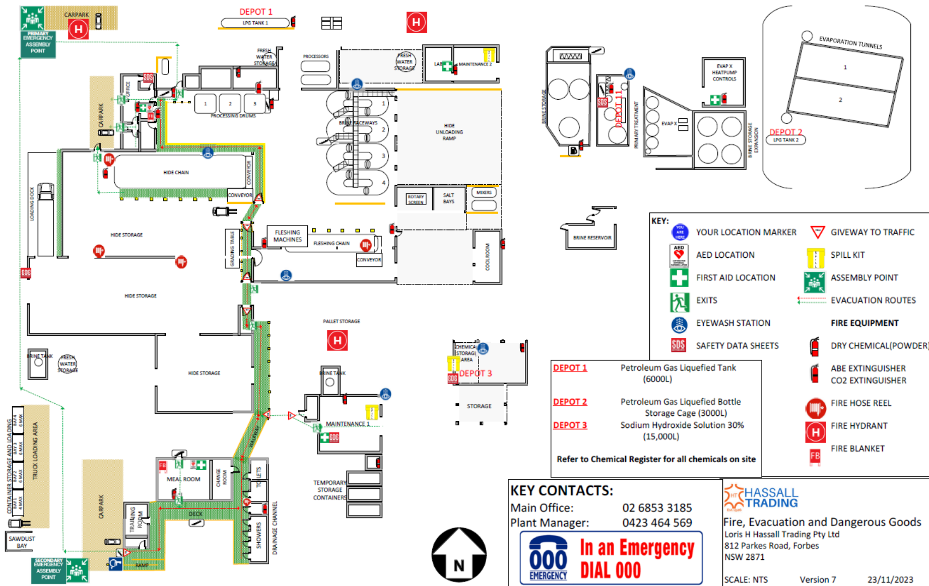
FIGURE 4: EMERGENCY EVACUATION SITE PLAN
