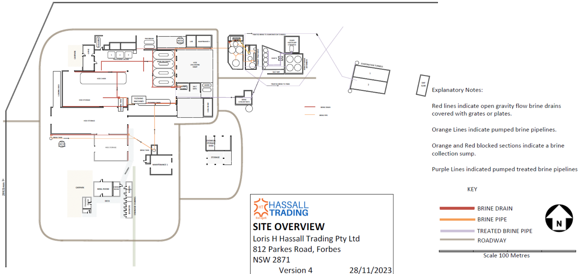
FIGURE 3: DRAINAGE SITE PLAN
